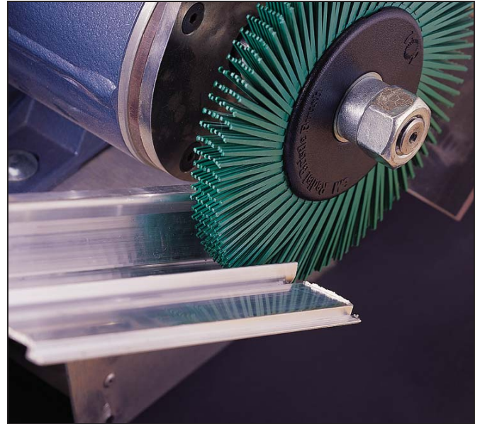
6" Deburring Aluminum Extrusion
